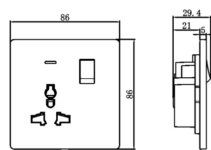
13A 1 gang switched MF socket, neon
