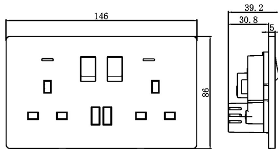
13A 2 gang DP switched socket+2 USB, neon
