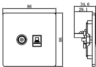
TV socket + data socket
