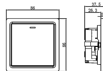
20A double pole switch with neon
