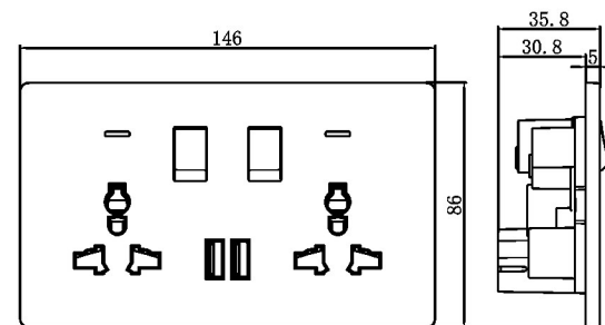
13A 2 gang switched MF socket+2USB, neon
