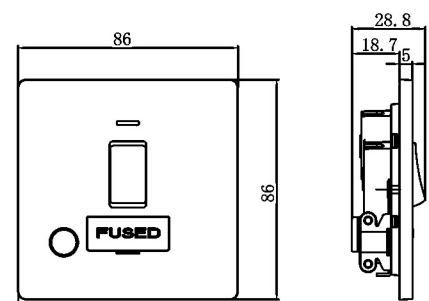
13A 1 gang switched fused connection unit, neon
