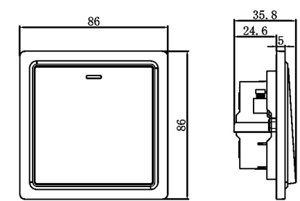
45A double pole switch with neon
